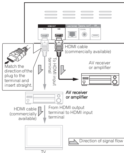
BDP-450's rear panel
