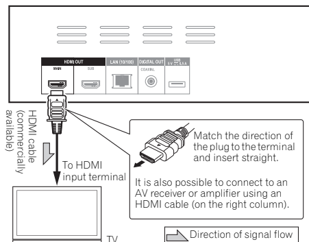
BDP-450's rear panel
